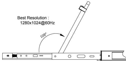
Figure 3-4 open angel of the console
