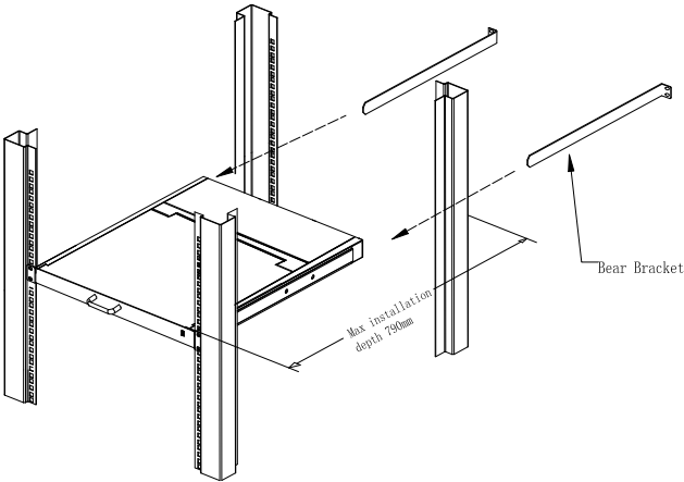
2-1 rack mounting (1)
